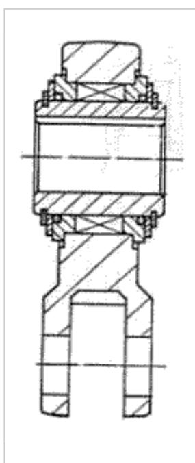
SPECIAL FREEWHEEL FOR PICKUP TRAILER
