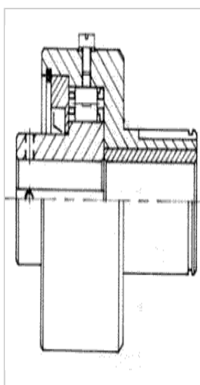
SPRAG CLUCH WITH STEEVE BEARING
