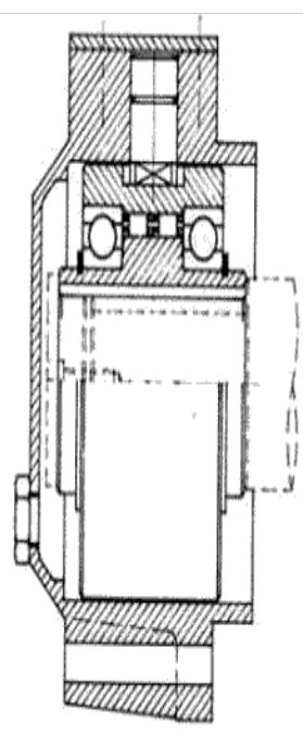
SPRAG TYPE BACKSTOP WITH BALL BEARING FOR GEAR-BOX APPLICATIONS
