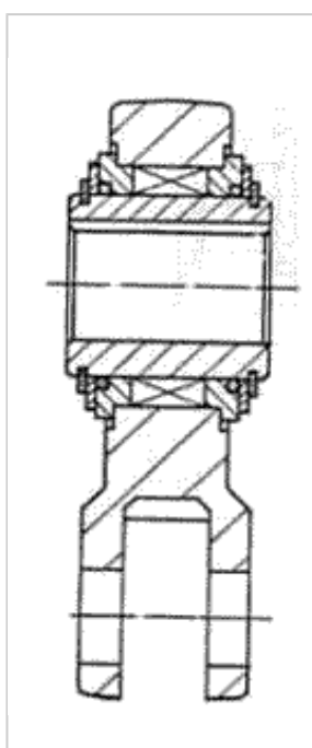
SPRAG FREEWHEEL FOR PICKUP TRAILER
