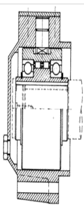
SPRAG TYPE BACKSTOP WITH BAND BEARING FOR GEAR BOX APPLICATION
