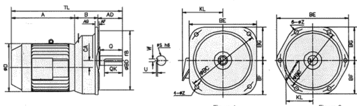
TYPE AVT-3 PHASE GEARMOTOR DIMENSIONS TABLE
