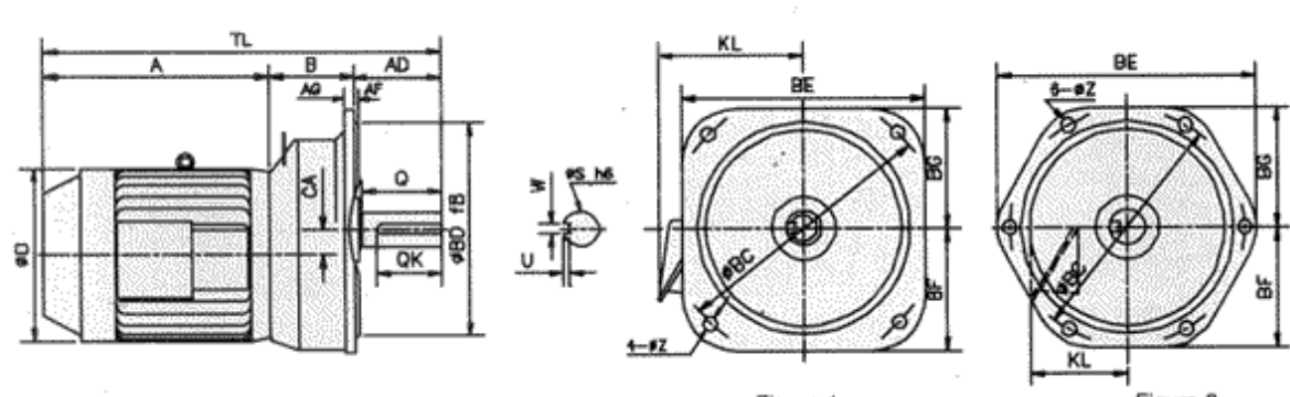
TYPE AVT-3 PHASE GEARMOTOR DIMENSIONS TABLE
