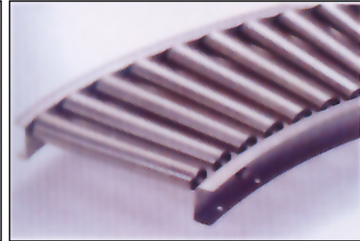
Taper Roller Conveyor
