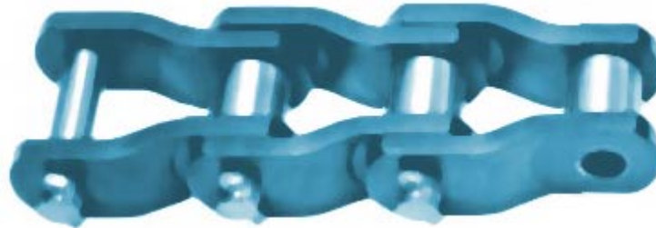
Type B Cranked Sidebars
